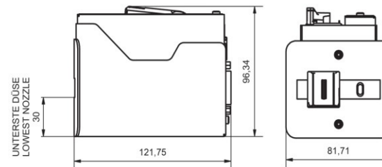
Dimension drawing technical data
